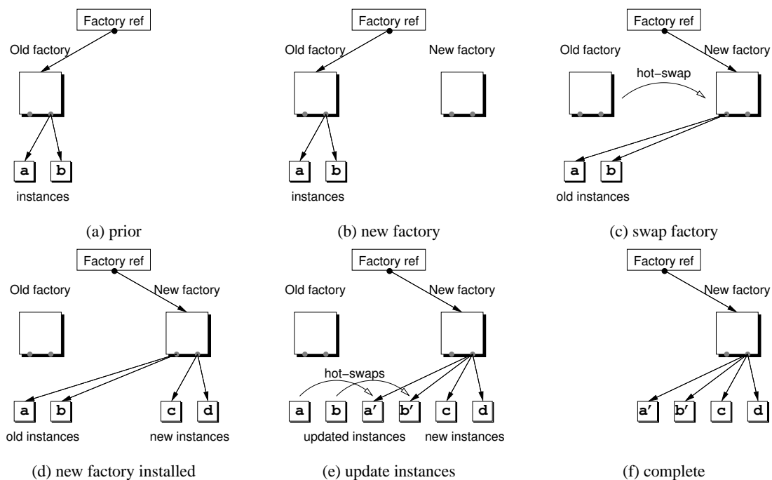
Figure 2: Phases in the dynamic update of a multiple-instance object: (a) prior to update the old factory is maintaining instances of a class; (b) instantiate a new factory for the updated class; (c) hot-swap the factory with its replacement (transferring the set of managed instances); (d) after the hot-swap, new instantiations are handled by the updated factory code (thus creating objects of the new type); (e) update old instances by hot-swapping each to an updated replacement; (f) the update is complete.
